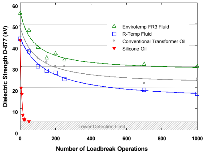
Fluid Loadbreak Dielectric Strength Retention Comparison
